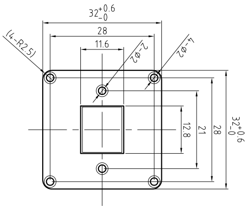
I/O Connector (12512WS-12B/Yeonho)
